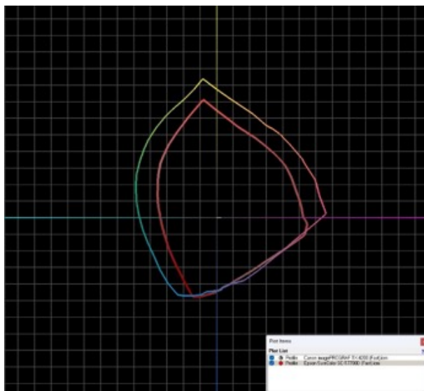
Canon imagePROGRAF TX-4200 colour gamut on plain paper in Fast settings (shown chromatically) vs. Epson SureColor SC-T7700D colour gamut (shown in red) on plain paper in Speed settings.
