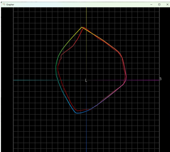
Canon TM-610M colour gamut on plain paper in High settings (shown chromatically) versus HP T850 MFP colour gamut (shown in red) on plain paper in Best settings.
