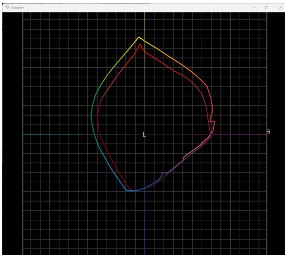
Canon TM-610M colour gamut on matte coated paper in High settings (shown chromatically) versus Epson SC-T5400M colour gamut (shown in red) on matte coated paper in Max Quality settings.
