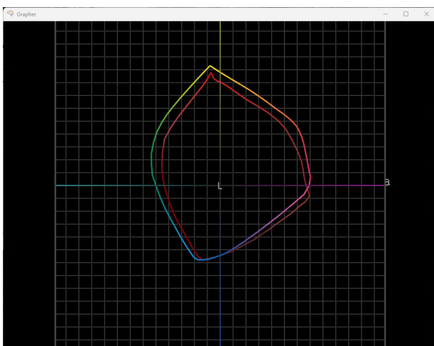
Canon TM-610M colour gamut on plain paper in High settings (shown chromatically) versus Epson SC-T5400M colour gamut (shown in red) on plain paper in Max Quality settings.
